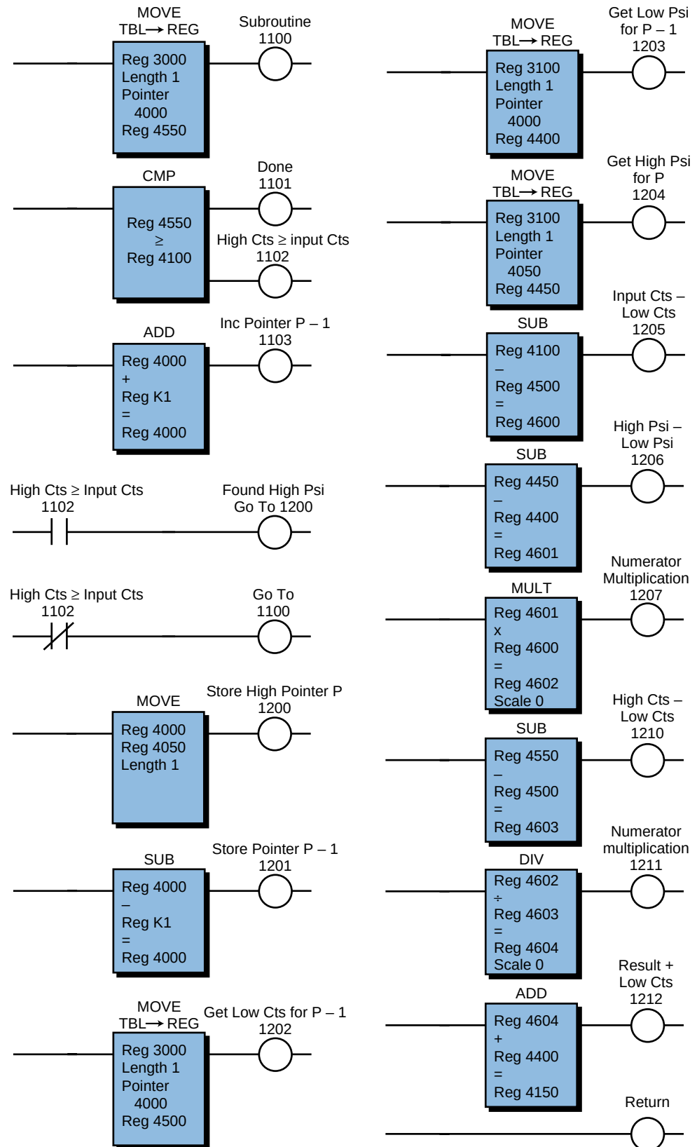
Figure 11-66. Interpolation subroutine.
