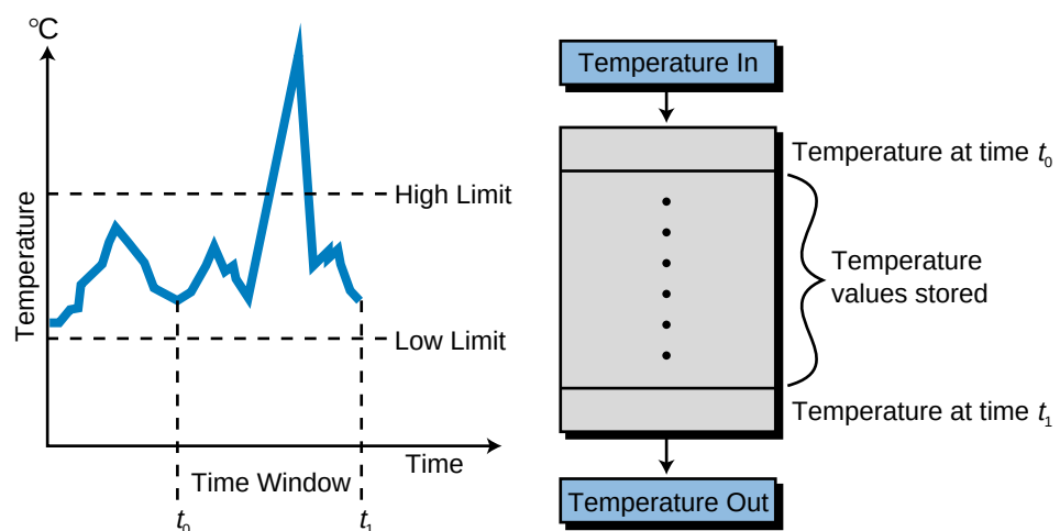
Figure 9-109. Temperature profile.
