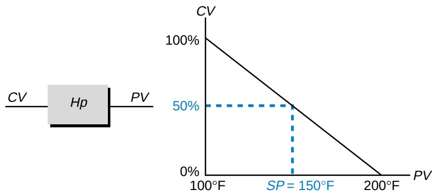
Figure 15-5. Process variable's reaction to a direct-acting controller.
