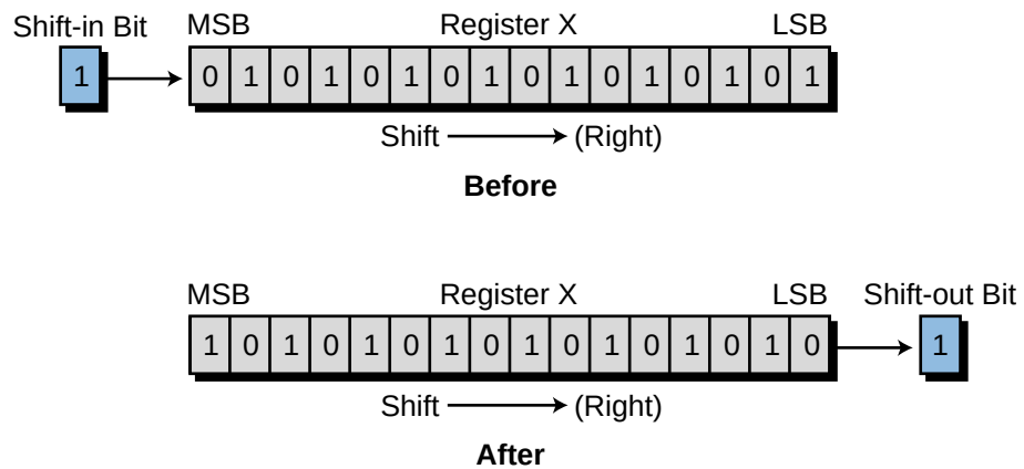
Figure 9-91. Right-shift execution.
