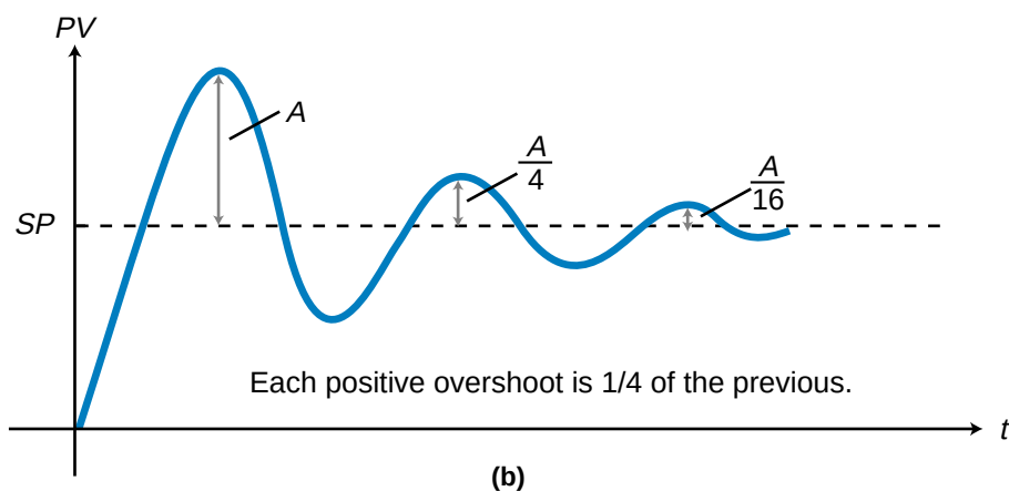
Figure 15-77. Process variable responses: (a) overdamped, critically damped, underdamped, and (b) quarter-amplitude.
