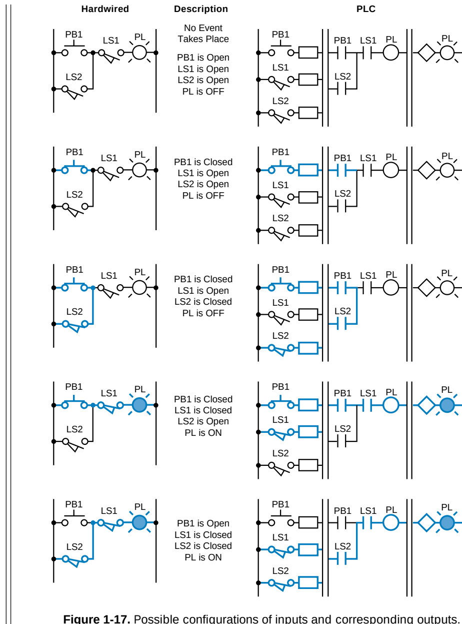
Figure 1-17. Possible configurations of inputs and corresponding outputs.
