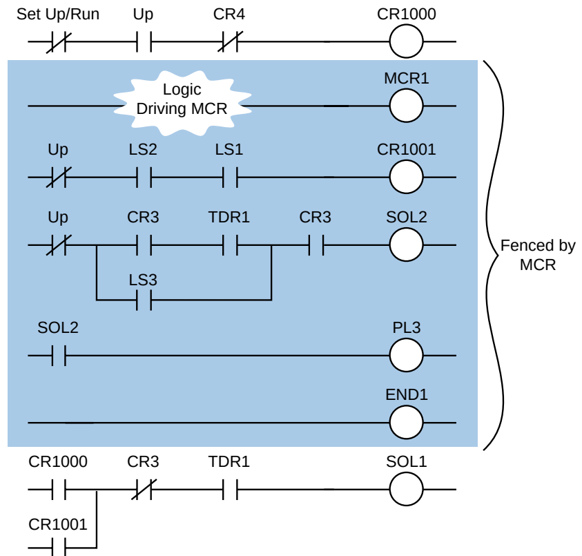
Figure 11-18. MCR fence.
