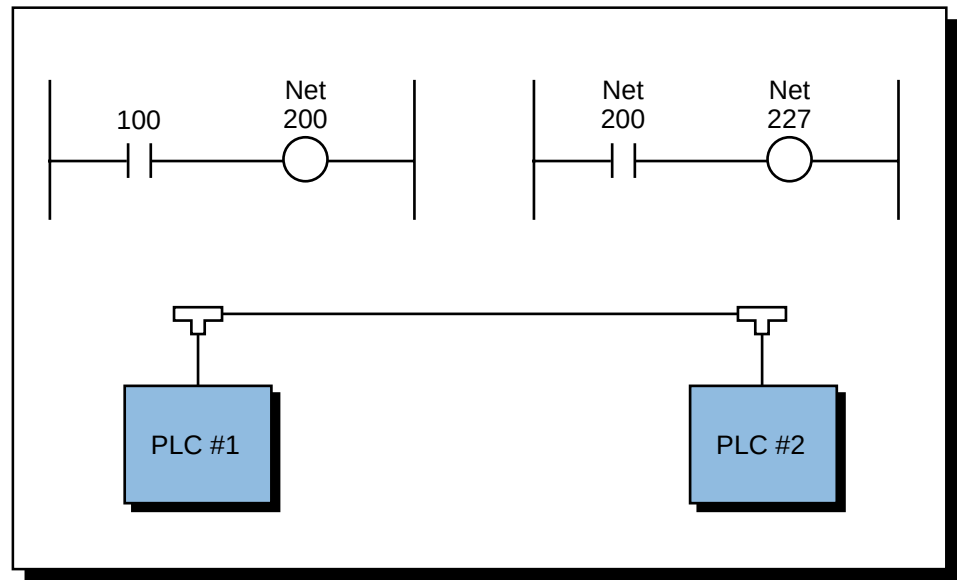
Figure 18-13. Network coils and contacts.
