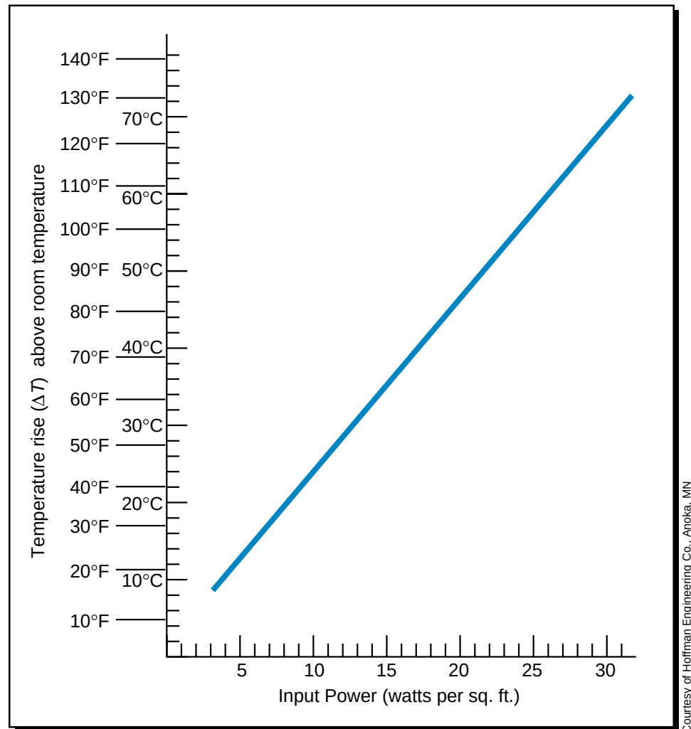
Figure 20-14. Temperature rise graph for a NEMA 12 enclosure.
