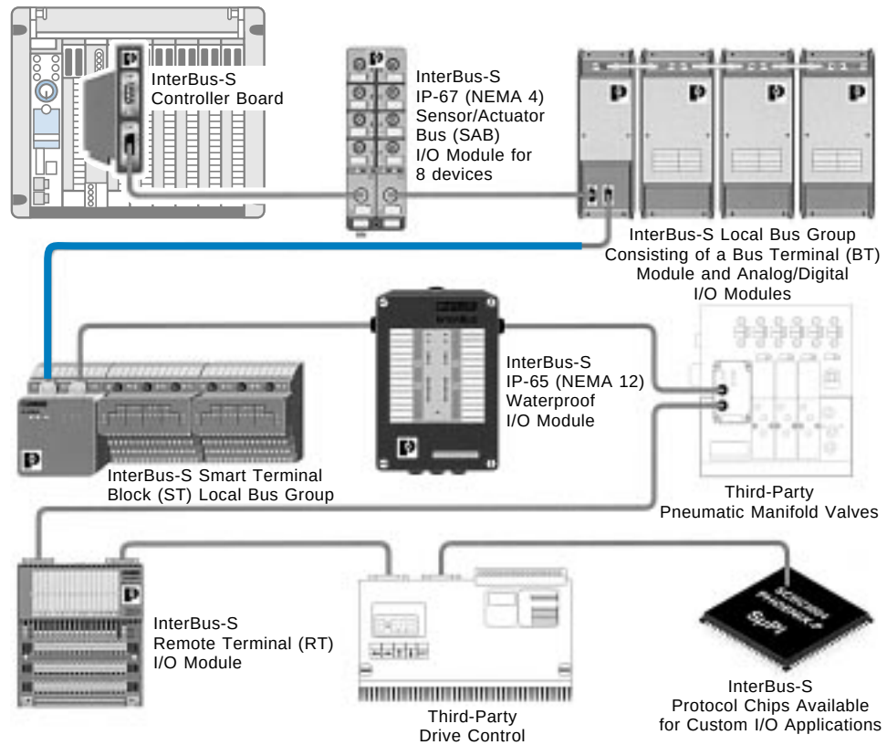
Figure 19-9. An InterBus-S network with a host controller interface to a PLC.
