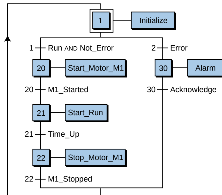
Figure 10-51. An alarm circuit with an OR divergence and an OR convergence.
