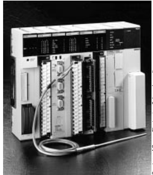
Figure 21-5. Omron's area B CV500 PLC with a temperature control module (up to 1024 I/O).
