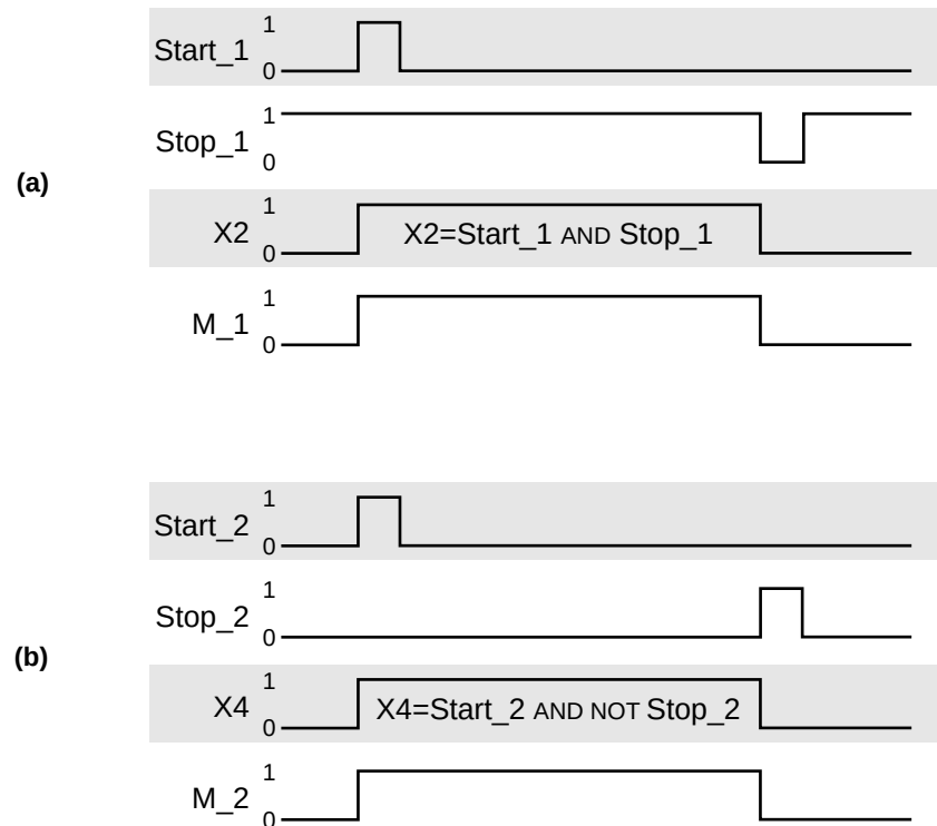
Figure 10-45. Timing diagrams for (a) Motor_1 and (b) Motor_2.
