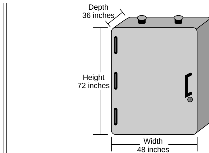
Figure 20-15. NEMA 12 enclosure.
