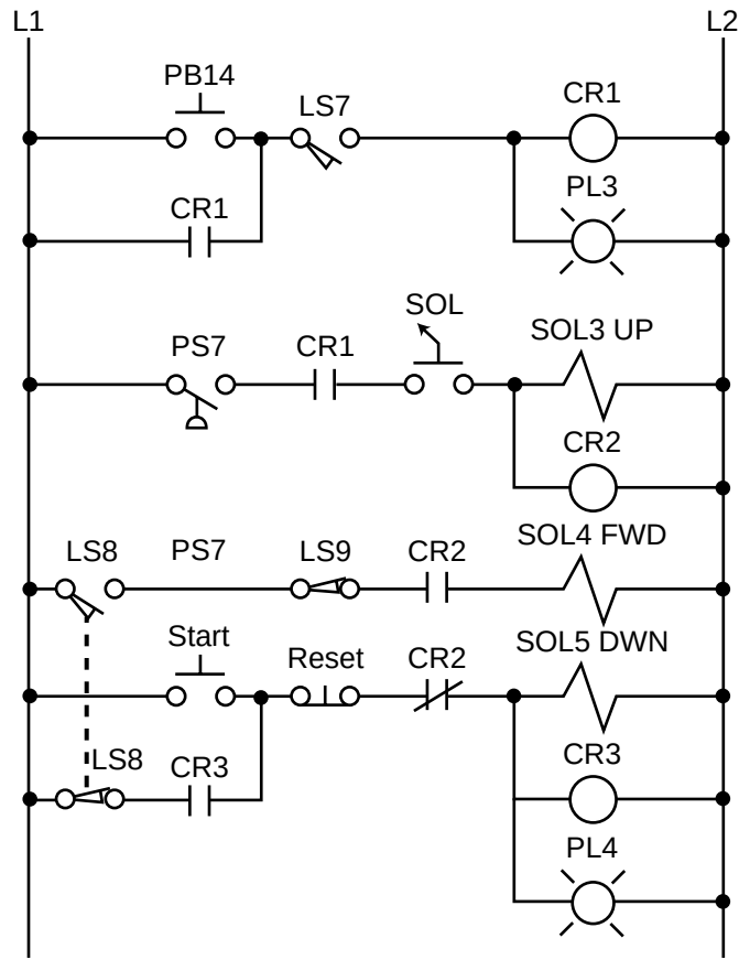
Figure 11-1. Electromechanical relay circuit diagram.
