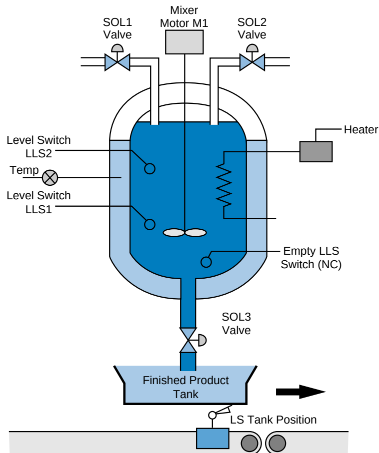
Figure 11-67. Process flow diagram of the batching application.
