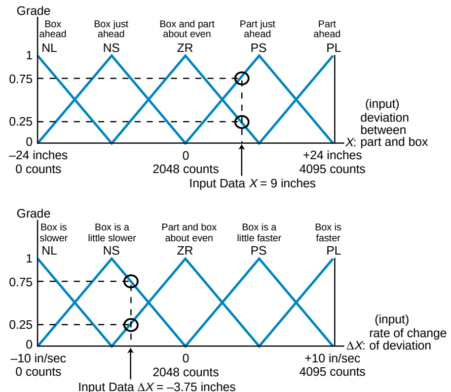
Figure 17-51. Part/box input membership functions.
