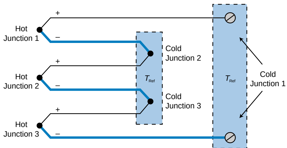
Figure 13-20. Thermopiling arrangement.
