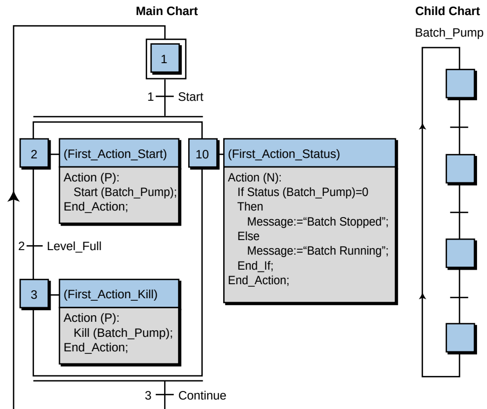
Figure 10-78. An SFC action programmed using ST and alternative SFC action syntax.
