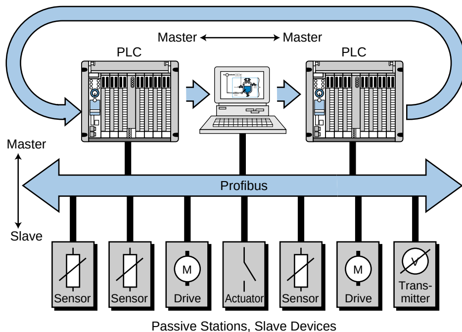
Figure 19-31. Master-slave and master-master Profibus communications.
