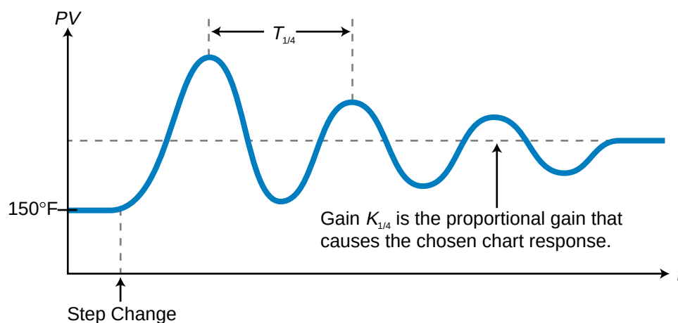
Figure 15-87. Quarter-amplitude test.
