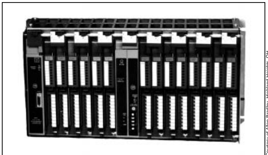
Figure 6-2. Typical discrete input/output system.
