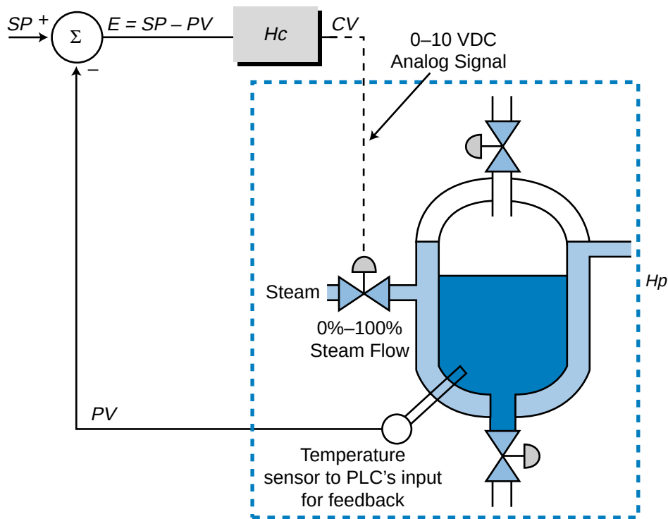
Figure 15-23. Block diagram of a continuous-mode controller.
