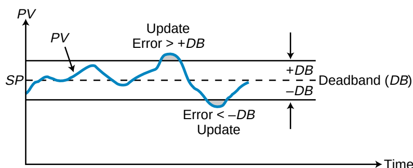
Figure 8-17. Error deadband.
