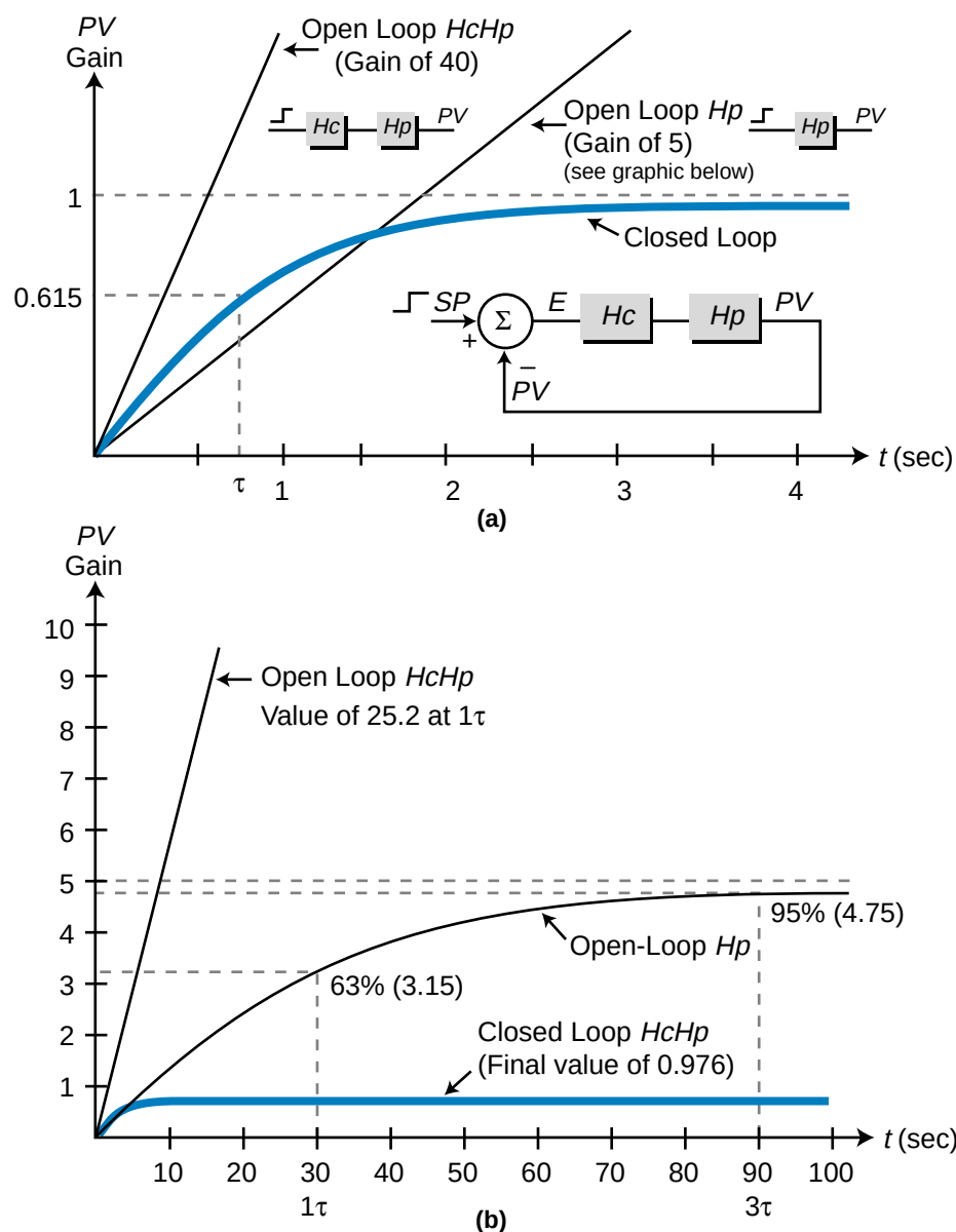
Figure 15-36. Open- and closed-loop responses shown in (a) detail and (b) 10× detail.
