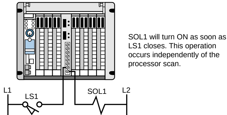
Figure 8-7. Fast-response interface.
